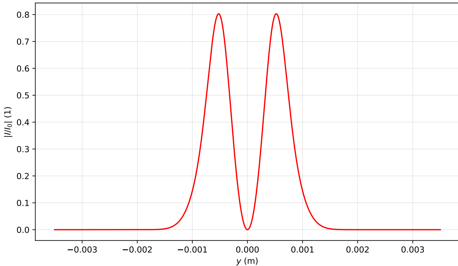
Intensity profile I(x=0, y, z=0.557)/I_0 , P_{in}=2.0P_{cr} , artificial time
